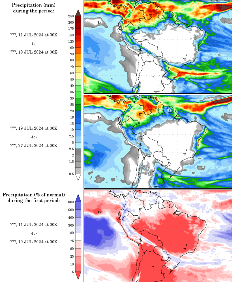
Precipitation forecasts from the National Centers for Environmental Prediction. Normal rainfall derived from Xie-Arkin (CMAP) Monthly Climatology for 1979-2003. Forecast Initialization Time: 00Z11JUL2024
