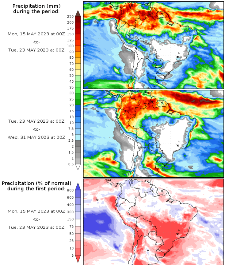
Precipitation forecasts from the National Centers for Environmental Prediction. Normal rainfall derived from Xie-Arkin (CMAP) Monthly Climatology for 1979-2003. Forecast Initialization Time: 00Z15MAY2023
